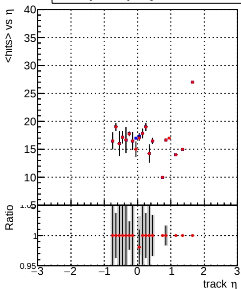
mean hits vs \eta Legend: DQM_CKF_QCDHighPt_base (blue line with markers), DQM_CKF_QCDHighPt_retrainOldFiles125_v2_prelimWPM_epoch1 (red line with markers)
