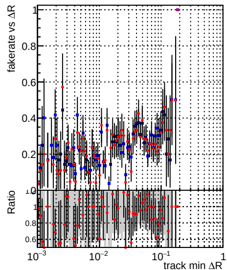
■ DQM_CKF_QCDHighPt_base ● DQM_CKF_QCDHighPt_retrainOldFiles125_v2_prelimWPM_epoch1
