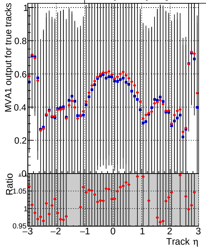
MVA1 of associated tracks (recoToSim) vs. track \eta Legend: ■ DQM_CKF_QCDHighPt_base ◆ DQM_CKF_QCDHighPt_retrainOldFiles125_v2_prelimWPM_epoch1
