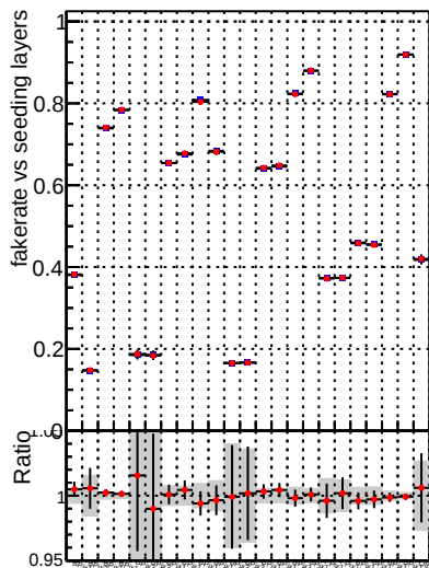
Fake rate vs. —•— DQM_CKF_QCDHighPt_base —•— DQM_CKF_QCDHighPt_retrainOldFiles125_v2_prelimWPM_epoch1
