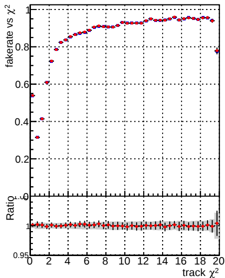
Fake rate vs. —•— DQM_CKF_QCDHighPt_base —•— DQM_CKF_QCDHighPt_retrainOldFiles125_v2_prelimWPM_epoch1
