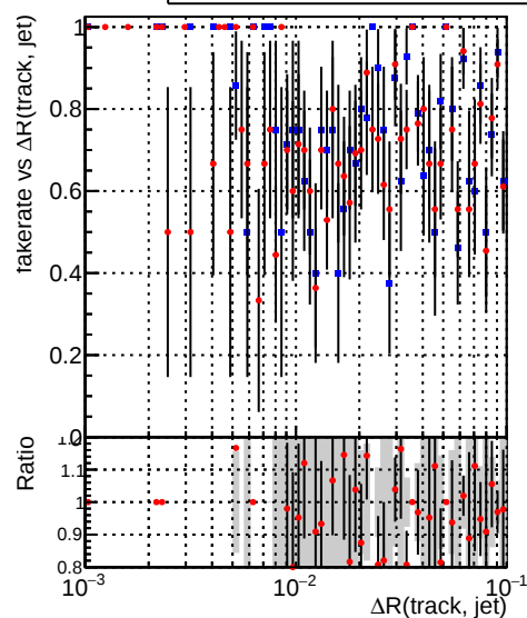
—●— DQM_CKF_QCDHighPt_base —●— DQM_CKF_QCDHighPt_retrainOldFiles125_v2_prelimWPM_epoch1
