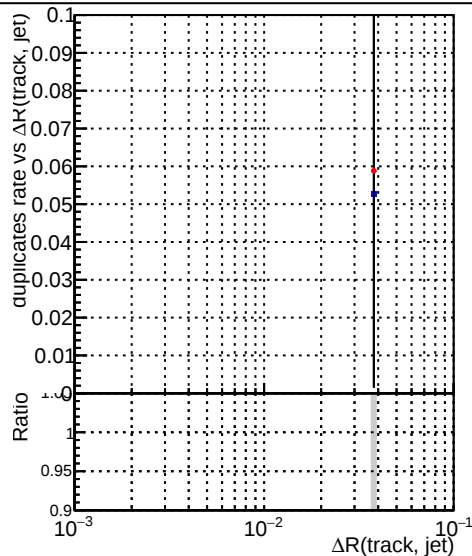
—●— DQM_CKF_QCDHighPt_base —●— DQM_CKF_QCDHighPt_retrainOldFiles125_v2_prelimWPM_epoch1
