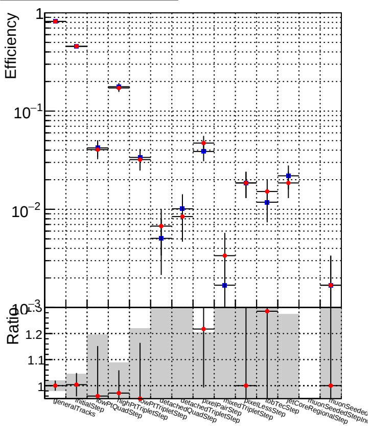
DQM_CKF_QCDHighPt_base DQM_CKF_QCDHighPt_retrainOldFiles125_v2_prelimWPM_epoch1
