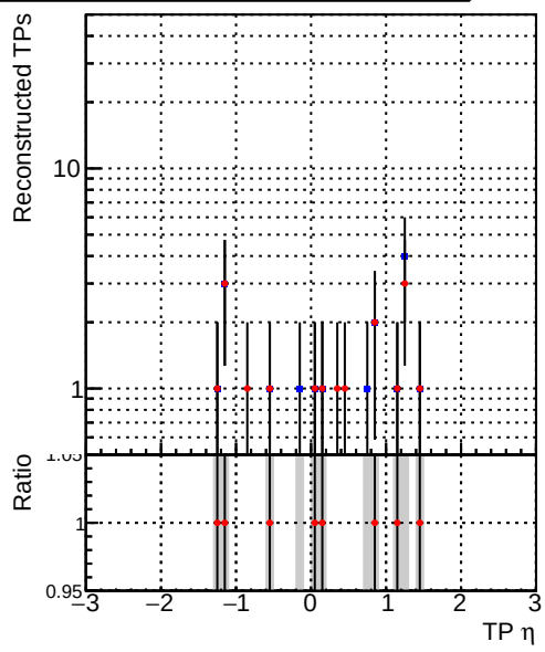
—●— DQM_CKF_QCDHighPt_base —●— DQM_CKF_QCDHighPt_retrainOldFiles125_v2_prelimWPM_epoch1
