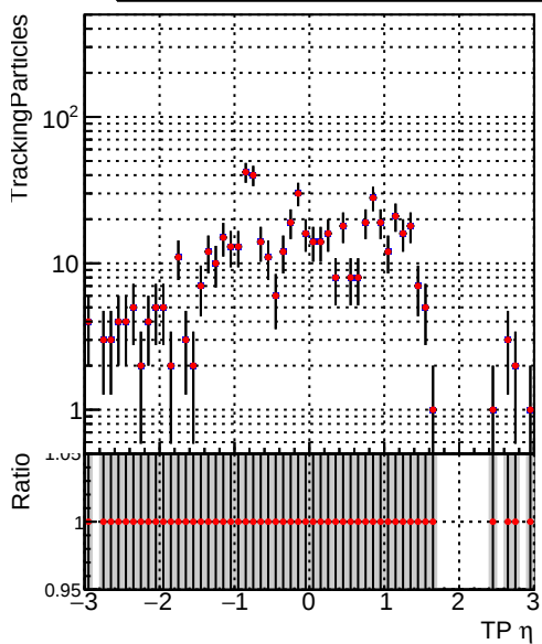
—•— DQM_CKF_QCDHighPt_base —•— DQM_CKF_QCDHighPt_retrainOldFiles125_v2_prelimWPM_epoch1
