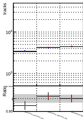
N of reco track vs. \chi^2 — DQM_CKF_QCDHighPt_base — DQM_CKF_QCDHighPt_retrainOldFiles125_v2_prelimWPM_epoch1
