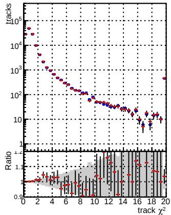
N of reco track vs. \chi^2 for DQM_CKF_QCDHighPt_base vs DQM_CKF_QCDHighPt_retrainOldFiles125_v2_prelimWPM_epoch1
