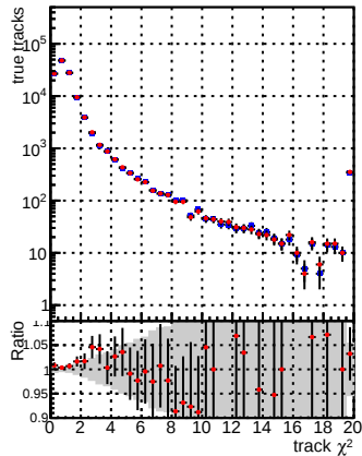
N of reco track vs. \chi^2 for DQM_CKF_QCDHighPt_base vs DQM_CKF_QCDHighPt_retrainOldFiles125_v2_prelimWPM_epoch1
