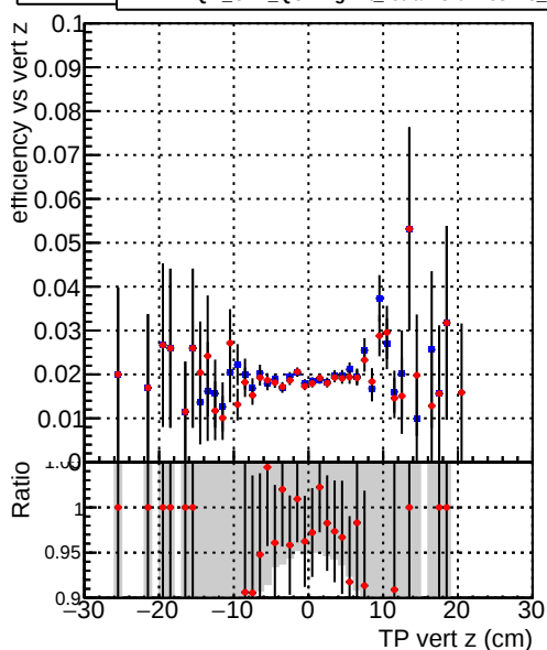
Efficiency — DQM_CKF_QCDHighPt_retrainOldFiles125_v2_prelimWPM_epoch1
