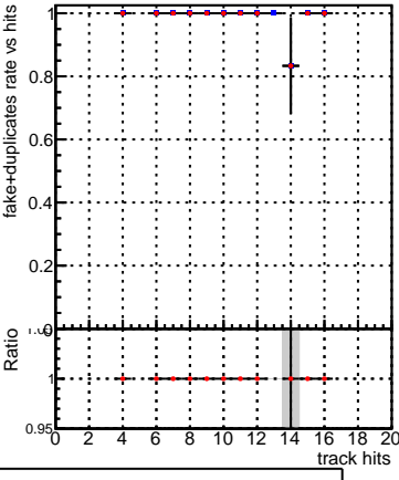
■ DQM_CKF_QCDHighPt_base ■ DQM_CKF_QCDHighPt_retrainOldFiles125_v2_prelimWPM_epoch1
