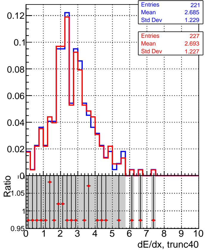
■ DQM_CKF_QCDHighPt_base ● DQM_CKF_QCDHighPt_retrainOldFiles125_v2_prelimWPM_epoch1
