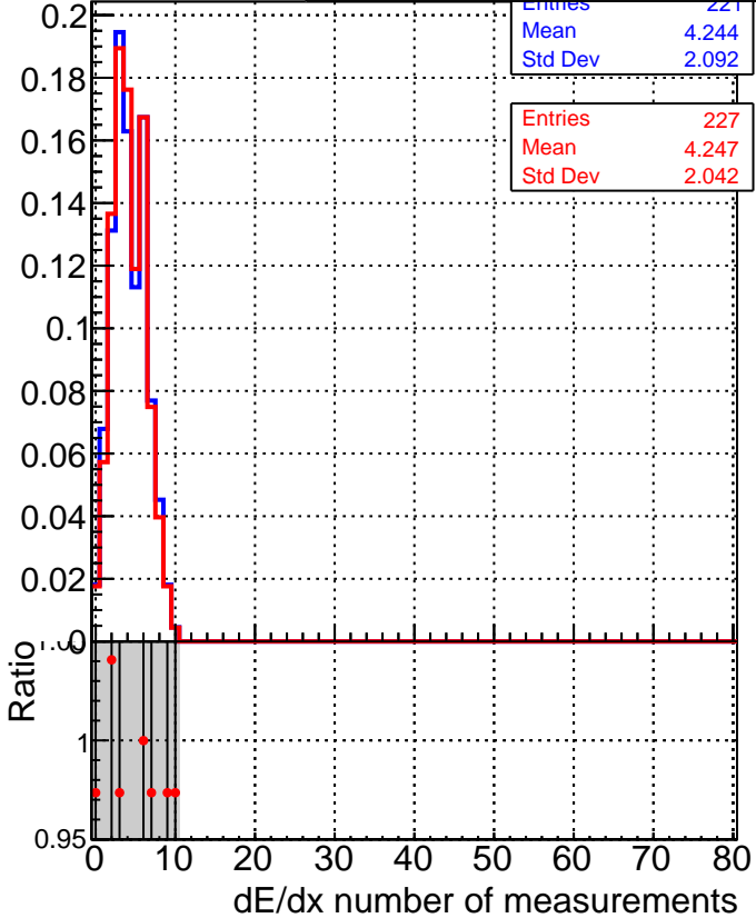
■ DQM_CKF_QCDHighPt_base ● DQM_CKF_QCDHighPt_retrainOldFiles125_v2_prelimWPM_epoch1
