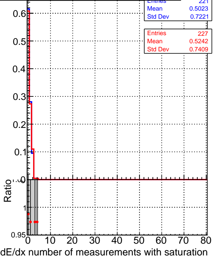
■ DQM_CKF_QCDHighPt_base ● DQM_CKF_QCDHighPt_retrainOldFiles125_v2_prelimWPM_epoch1
