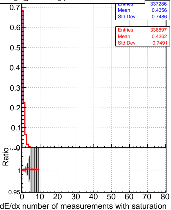
■ DQM_CKF_QCDHighPt_base ● DQM_CKF_QCDHighPt_retrainOldFiles125_v2_prelimWPM_epoch1
