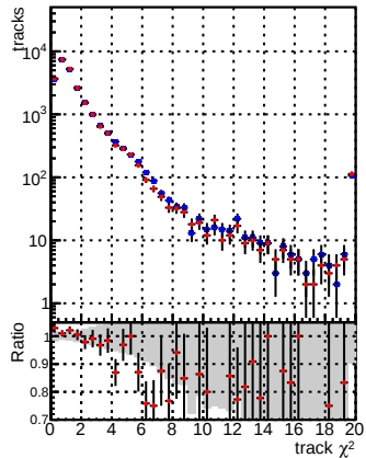
N of reco track vs. \chi^2 for DQM_CKF_QCDHighPt_base and DQM_CKF_QCDHighPt_retrainOldFiles125_v2_prelimWPM_epoch1
