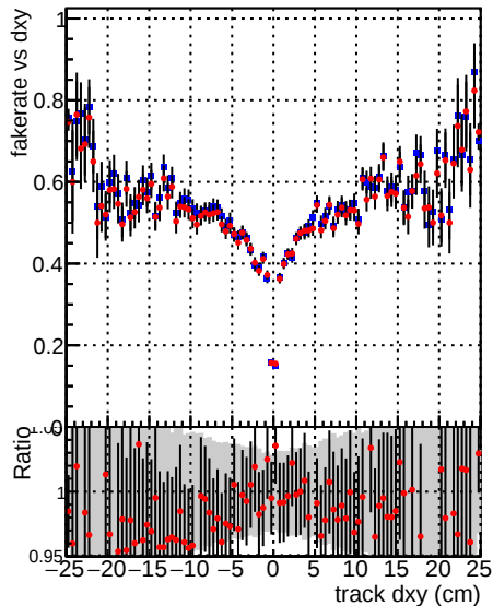
—●— DQM_CKF_QCDHighPt_base —●— DQM_CKF_QCDHighPt_retrainOldFiles125_v2_prelimWPM_epoch1
