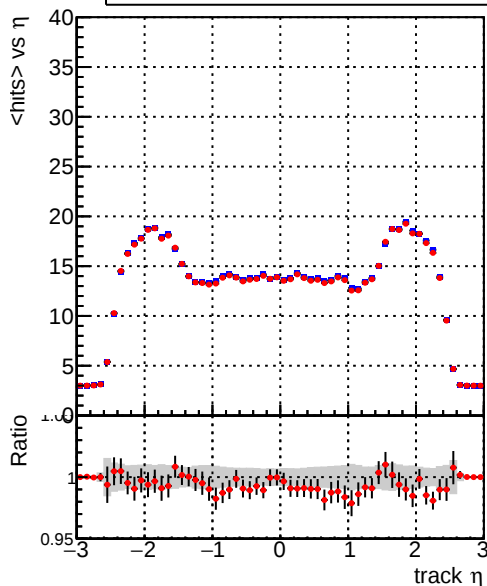
mean hits — DQM_CKF_QCDHighPt_base — DQM_CKF_QCDHighPt_retrainOldFiles125_v2_prelimWPM_epoch1
