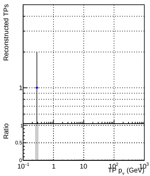
Legend: DQM_CKF_TT_retrain (blue dot), DQM_mkFit_TT_retrain (red dot)
