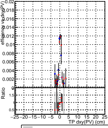
Efficiency vs DQM_CKF_TT_retrain (blue squares) and DQM_mkFit_TT_retrain (red circles)
