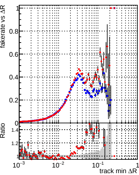
Fake rate vs \Delta R (track, jet) DQM_CKF_TT_retrain DQM_mkFit_TT_retrain
