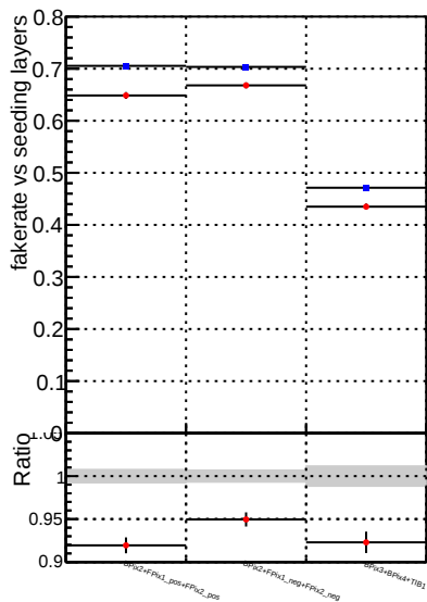
Fake rate vs. —●— DQM_CKF_TT_retrain —●— DQM_mkFit_TT_retrain
