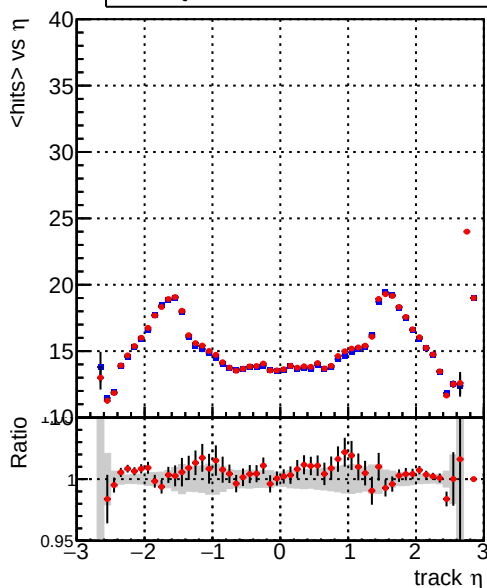
mean hits vs \eta Legend: DQM_CKF_TT_retrain (blue line), DQM_mkFit_TT_retrain (red line)
