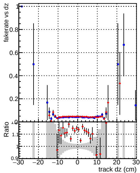
Fake rate vs dz —●— DQM_CKF_TT_retrain —●— DQM_mkFit_TT_retrain
