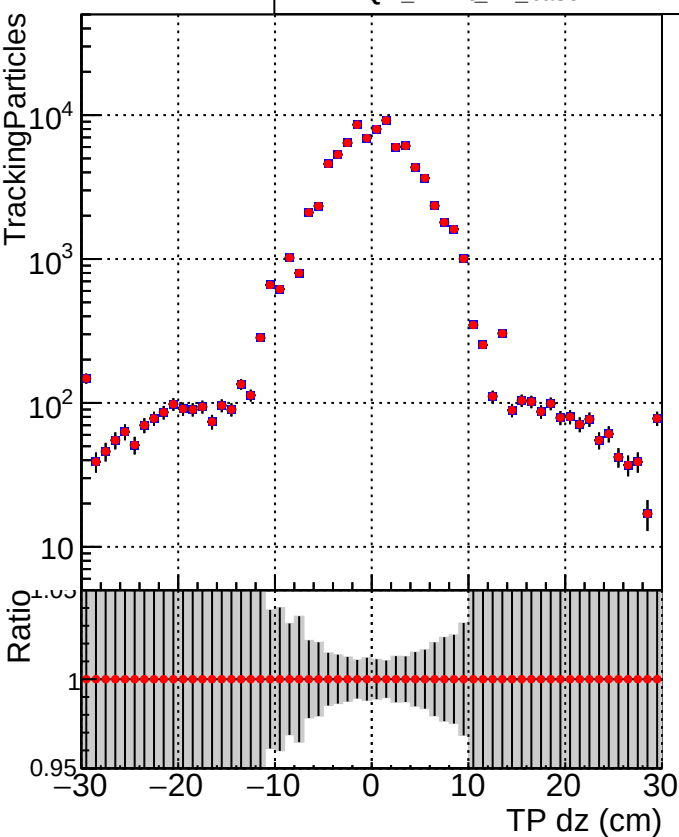
Legend: ■ DQM_CKF_TT_base ● DQM_mkFit_TT_base
