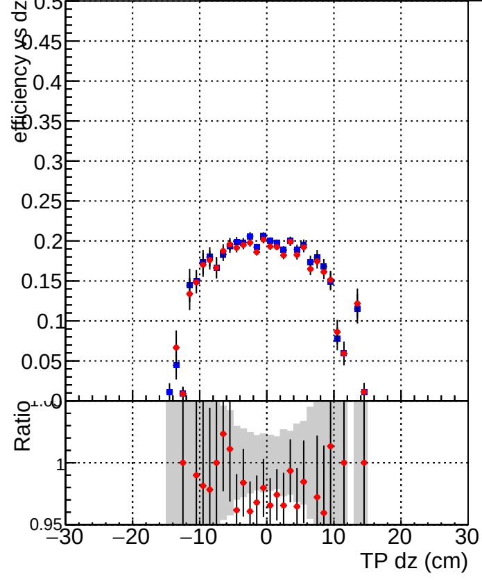
Efficiency vs Dz Legend: DQM_CKF_TT_base (blue square) DQM_mkFit_TT_base (red circle)
