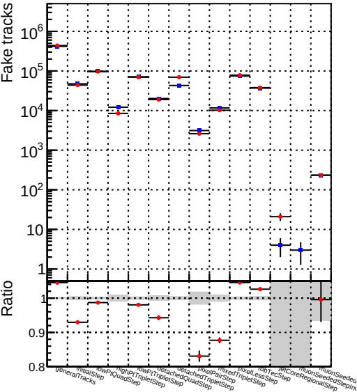
Number —●— DQM_mkFit_TT_base
