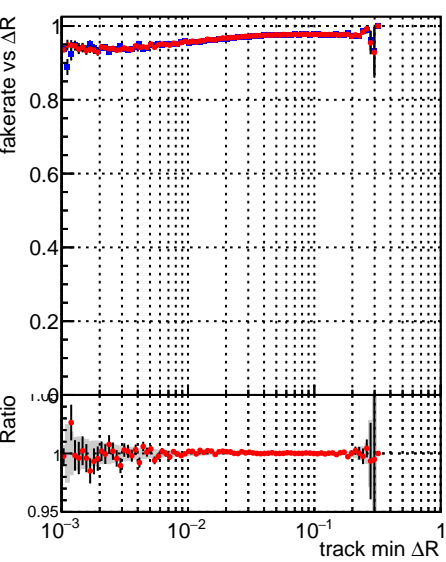
Fake rate vs \Delta R (track, jet) Legend: ■ DQM_CKF_TT_base, ● DQM_mkFit_TT_base
