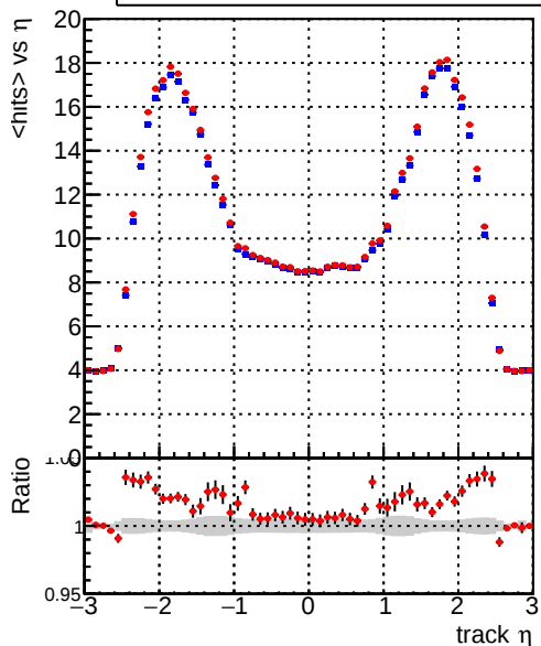
— DQM_CKF_TT_base — DQM_mkFit_TT_base mean hits
