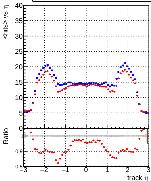
DQM_CKF_TT_base mean hits DQM_mkFit_TT_base
