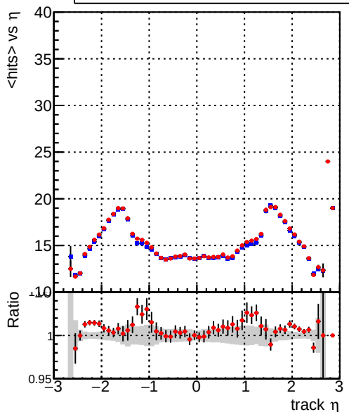
mean hits vs \eta Legend: DQM_CKF_TT_base (blue line), DQM_mkFit_TT_base (red line)
