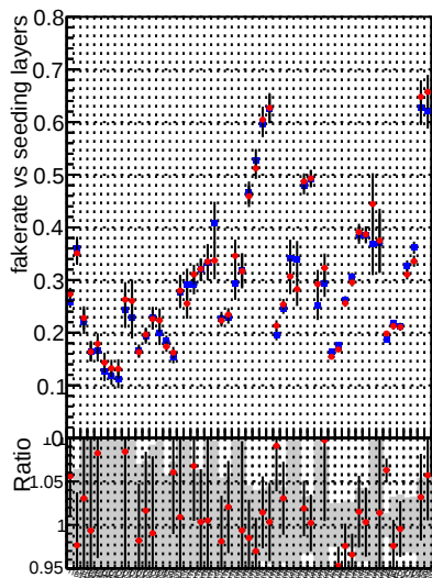
Fake rate vs. —◆— DQM_CKF_TT_base —▲— DQM_mkFit_TT_base
