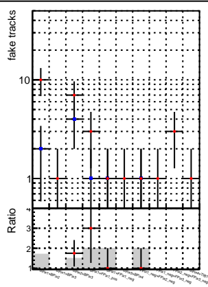
N of fake tracks vs. s
