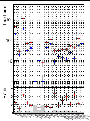
N of associated (recoToSim) tracks vs. s
