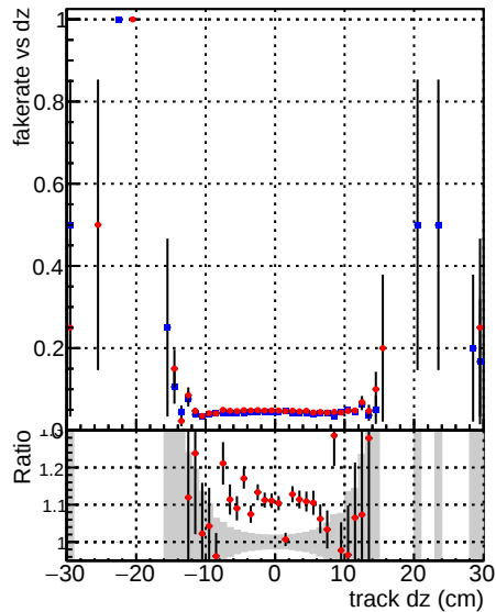
—●— DQM_CKF_TT_base —●— DQM_mkFit_TT_base
