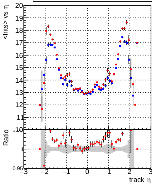
mean hits vs \eta Legend: DQM_CKF_TT_base (blue line), DQM_mkFit_TT_base (red line)
