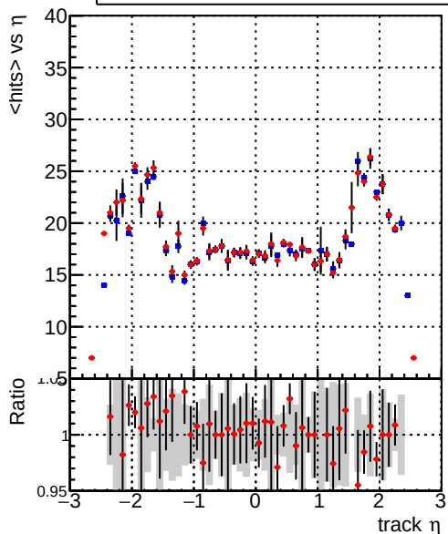
mean hits vs \eta — DQM_CKF_TT_base — DQM_mkFit_TT_base
