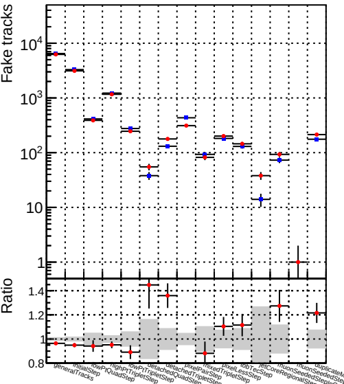
Number —●— DQM_mkFit_TT_base
