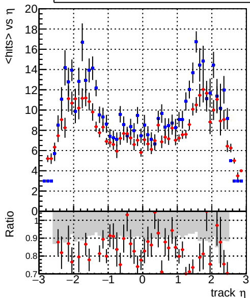
mean hit — DQM_CKF_TT_base — DQM_mkFit_TT_base
