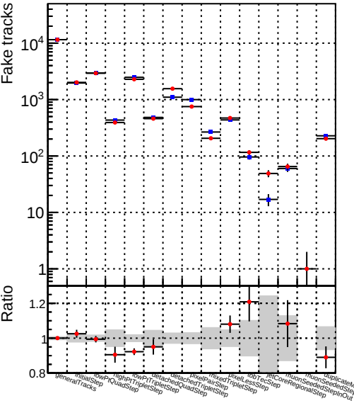
Number —●— DQM_mkFit_TT_base
