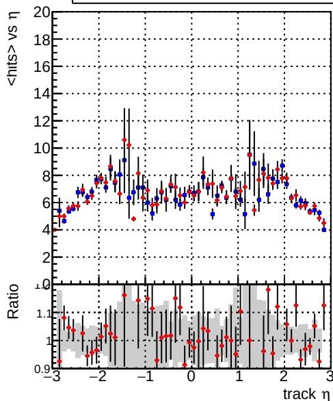
mean hits vs \eta Legend: DQM_CKF_TT_base (blue line with markers), DQM_mkFit_TT_base (red line with markers)
