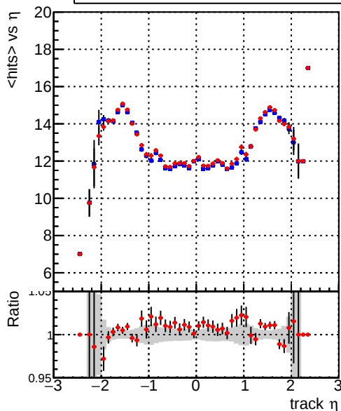
— DQM_CKF_TT_base — DQM_mkFit_TT_base mean hits vs \eta
