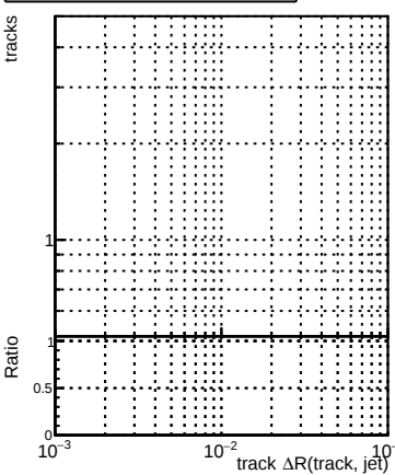
N of reconstructed tracks vs dR(track,jet)
