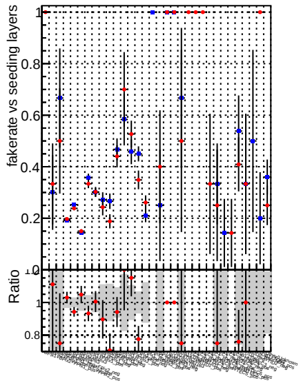
Fake rate vs. —•— DQM_CKF_TT_base —•— DQM_mkFit_TT_base
