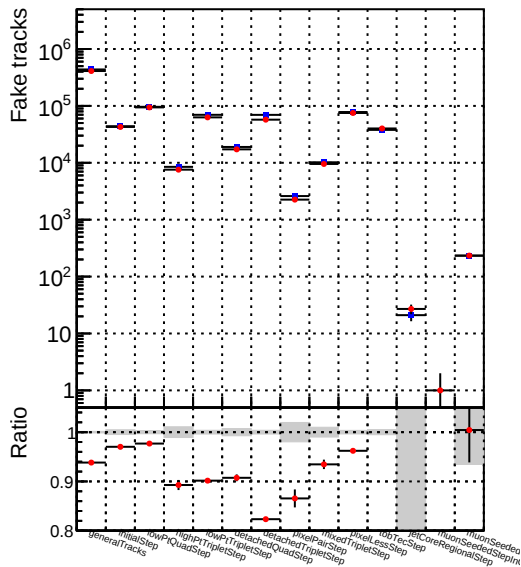
Number of tracks vs collection Legend: DQM_mkFit_TT_base (blue line with circles), DQM_mkFit_TT_retrain (red line with circles)
