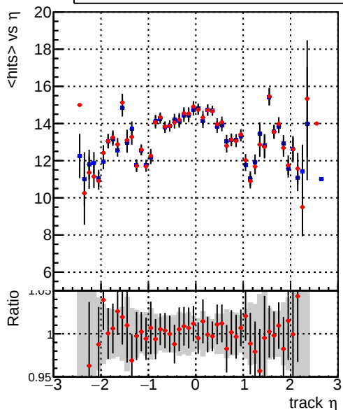
mean hits Legend: DQM_mkFit_TT_base (blue line), DQM_mkFit_TT_retrain (red line)
