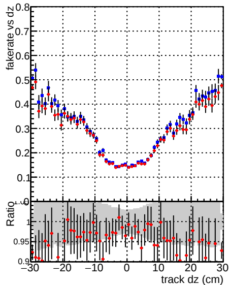
Fake rate vs dz —●— DQM_mkFit_TT_base —●— DQM_mkFit_TT_retrain
