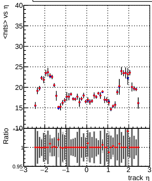
mean hit Legend: DQM_mkFit_TT_base (blue line), DQM_mkFit_TT_retrain (red line)
