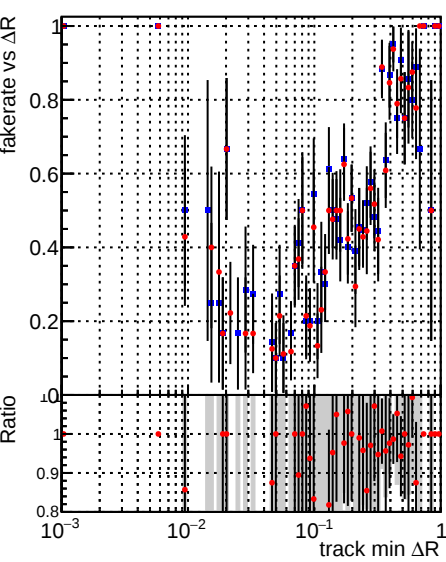
Fake rate vs \Delta R (track, jet) DQM_mkFit_TT_base DQM_mkFit_TT_retrain
