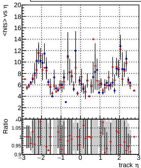
mean hit — DQM_mkFit_TT_base — DQM_mkFit_TT_retrain
