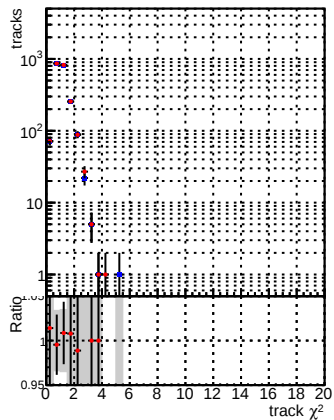
N of reco track vs. \chi^2 for DQM mkFit TT_base and DQM mkFit TT_retrain
