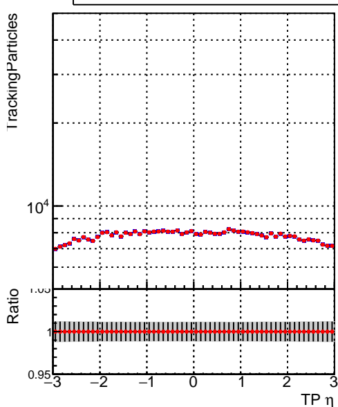
N of simulated tracks vs \eta — DQM_mkFit_TT_base — DQM_mkFit_TT_retrain
